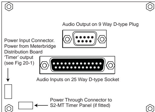
Fig 20-10b : S2-M6SS Diagram.
