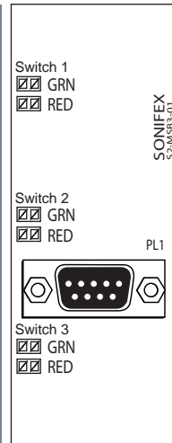
Fig 20-12b : S2-MSB3 Diagram.
