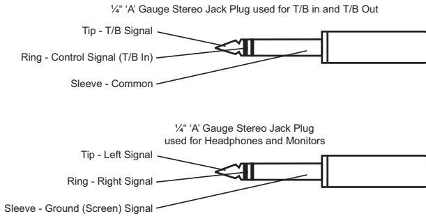
Fig 2-6 : 1/4" Jack Connectors.
